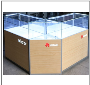
Name: corner showcase MEANS: 1200*450*600mm 450*450*600mm 1200*450*600mm accept custom size Material: stainless steel ,MDF , nature wood veneer, LED light Technology: detachable
